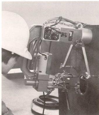
Cutting in vertical surfaces
