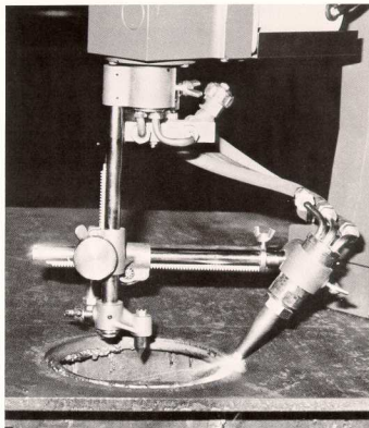
Bevel cutting
